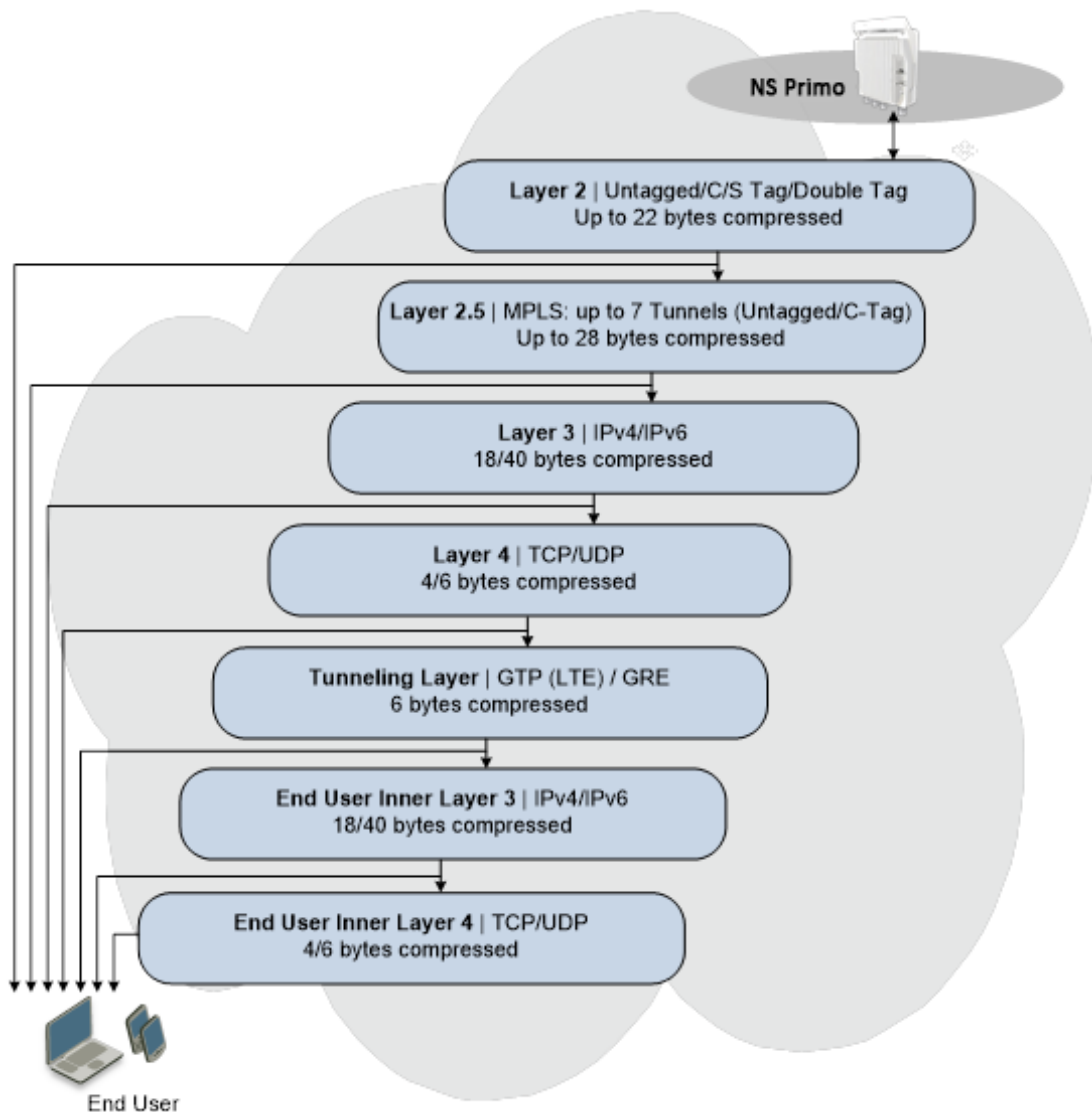
Header De-Duplication Potential Throughput Savings per Layer
