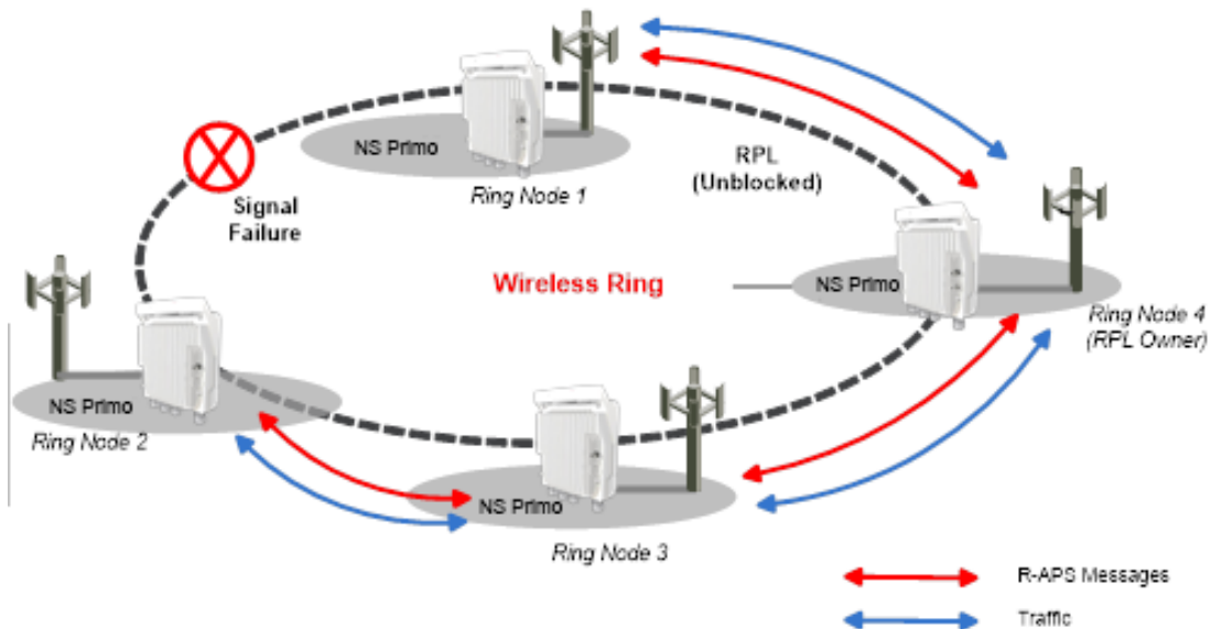
G.8032 Ring in Protecting State
