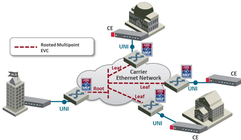
MEF Ethernet Private Tree Example
