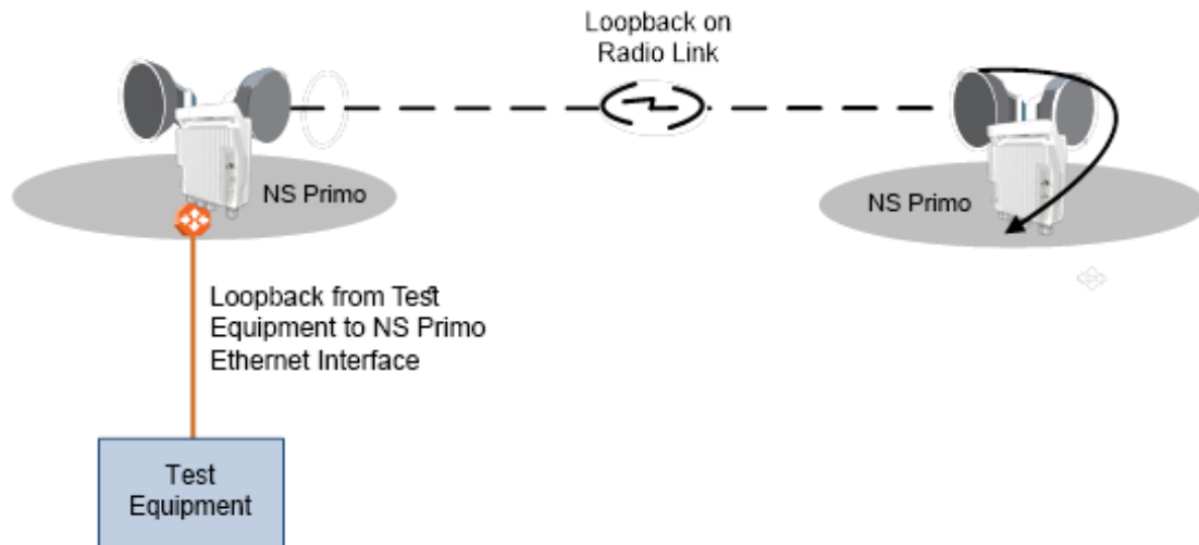
Ethernet Line Interface Loopback – Application Examples
