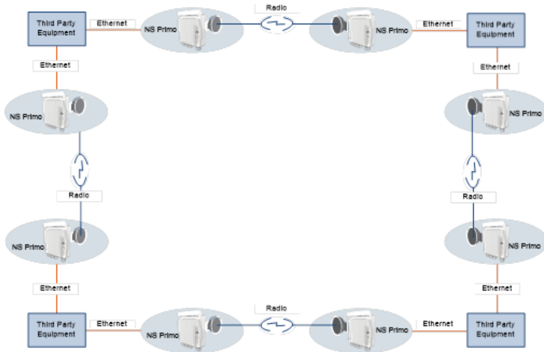
Network Topology with NetStream Primo Units and Third-Party Equipment
