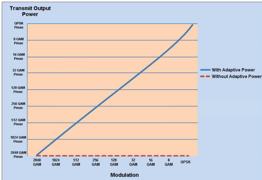
NetStream Primo ACM with Adaptive Power Contrasted to Other ACM Implementations
