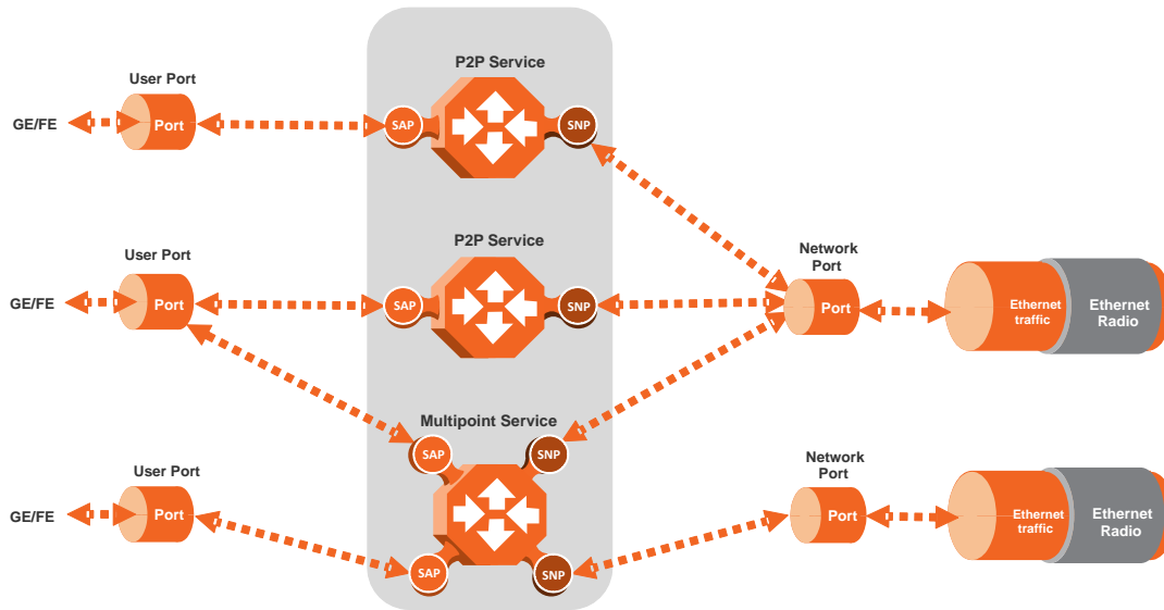
NetStream Primo Services Flow
