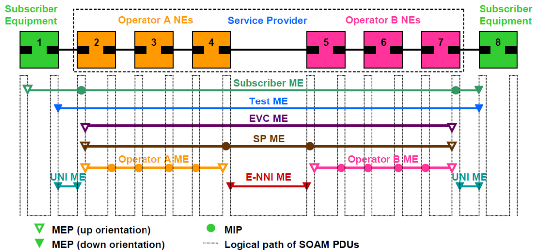
SOAM Maintenance Entities (Example)
