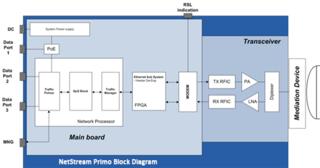
NetStream Primo Block Diagram
