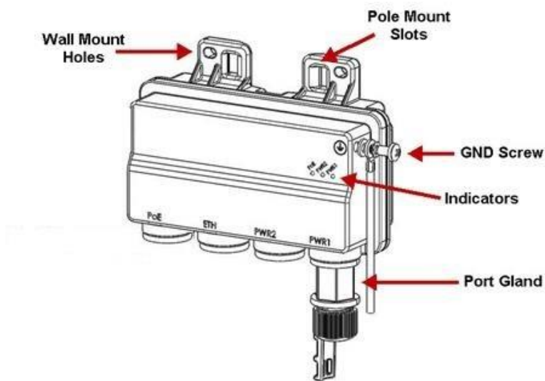
PoE Injector
