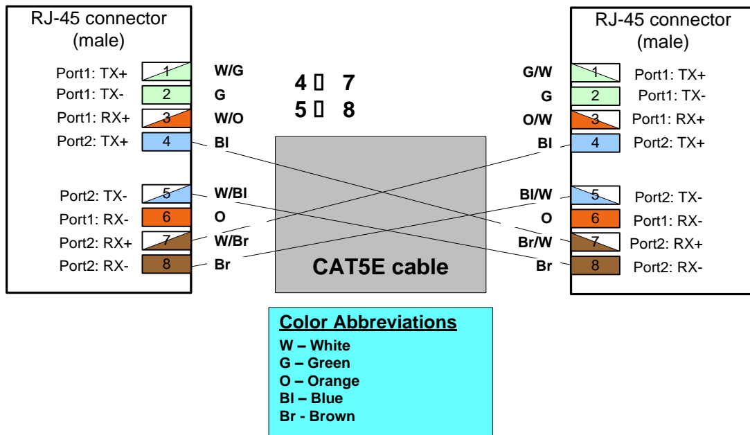
Protection Signaling Cable Pinouts
